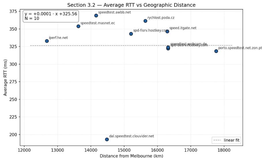
< Fig 3.2.14 Scatter chart (distance VS Avg RTT)>
